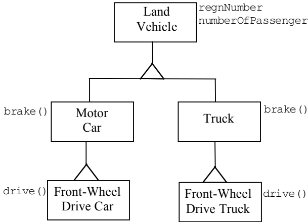
Figure 6-20: Front-Wheel Drive class as subclasses: representation scheme.
