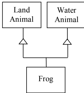
Figure 6-10: Multiple inheritance.
