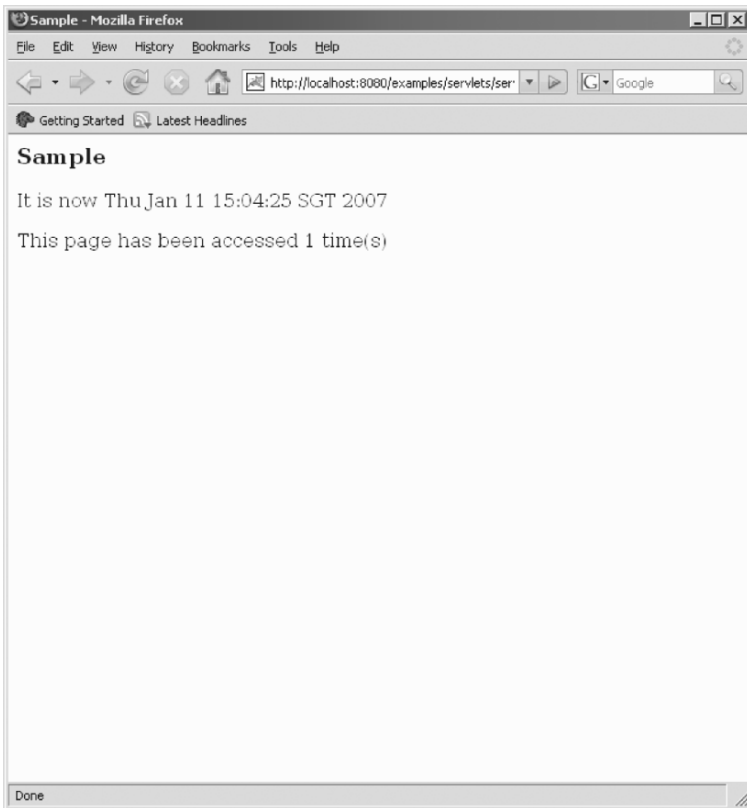
Figure 15-6: Servlet result.
