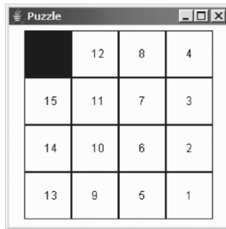
Figure 13-18: Puzzle board.
