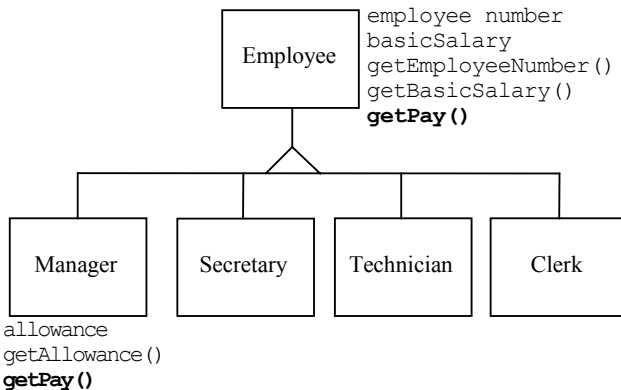
Figure 6-6: Redefining getPay() method of Manager .
