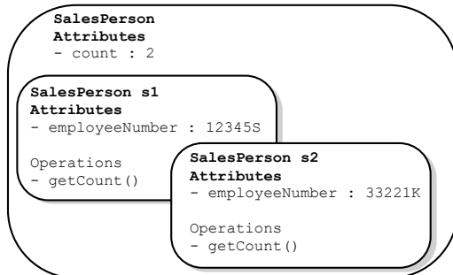
Figure 8-2: Shared variable count .
