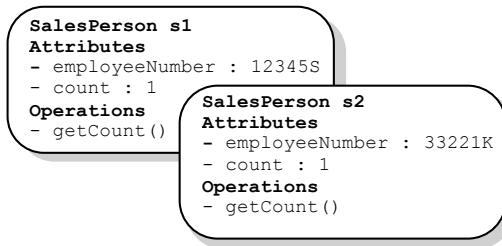
Figure 8-1: State of SalesPerson objects.
