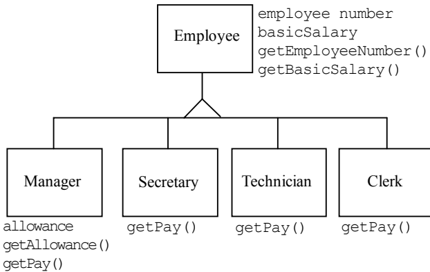
Figure 6-5: Extended Employee class hierarchy.
