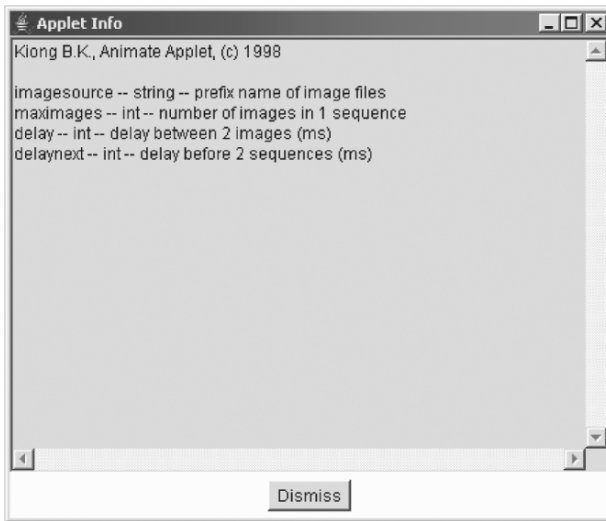
Figure 14-3: Applet information.
