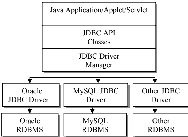
Figure 17-1: JDBC Architectural Stack.
