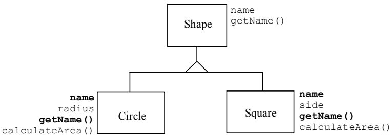
Figure 6-7: Class hierarchy of Shape, Circle and Square.
