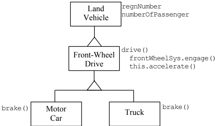
Figure 6-19: “Front-Wheel Drive Class as Superclass” Representation Scheme
