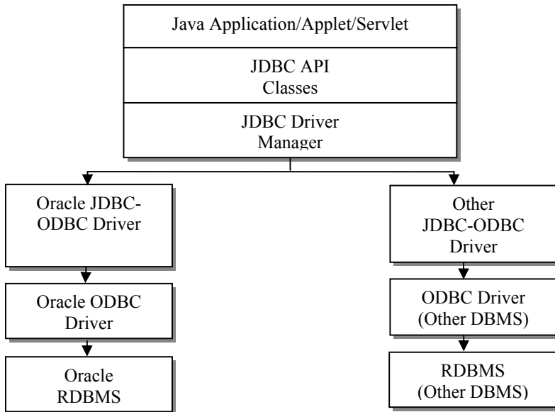
Figure 17-2: Type 1 JDBC drivers.
