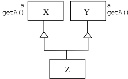
Figure 6-13: Redefined attribute and method in multiple inheritance paths.
