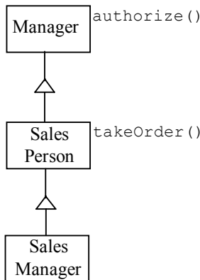
Figure 6-12: A SalesManager class hierarchy using single inheritance.
