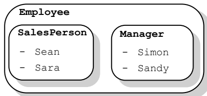
Figure 5-2: Employee, SalesPerson and Manager classes.
