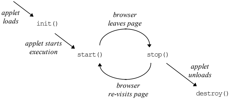
Figure 14-2: Applet life-cycle.
