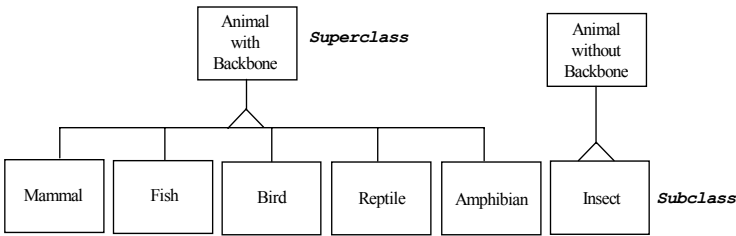
Figure 5-4: Generalizing classes.
