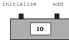
Figure 2-2: A counter.
