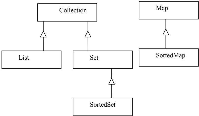
Figure 12-1: Java Collections Framework’s core interfaces.
