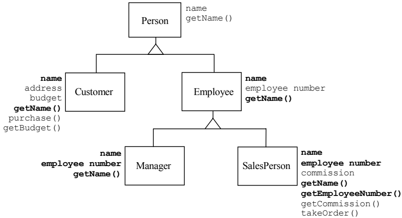
Figure 6-2: Classes with inherited properties.
