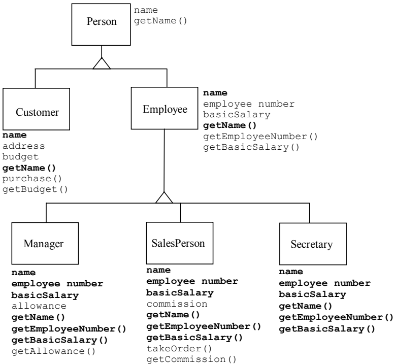
Figure 6-3: Including the Secretary class.
