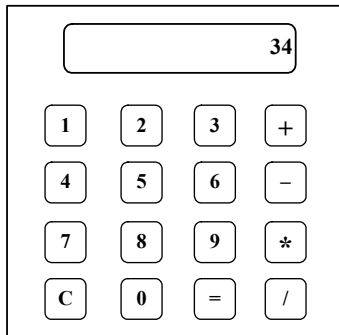
Figure 4-1: Four-function calculator.
