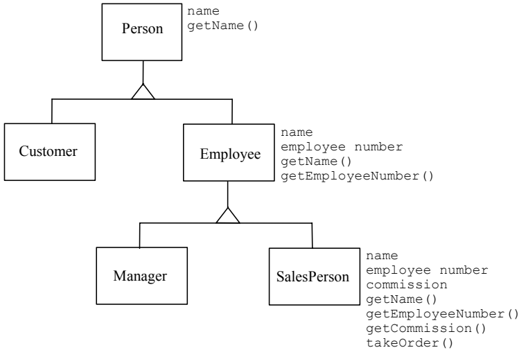
Figure 6-1: Common properties in classes.
