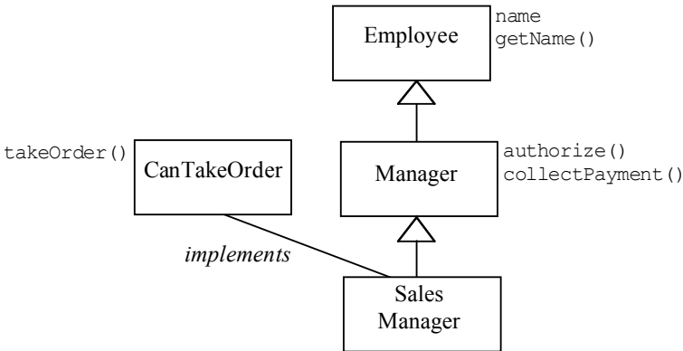
Figure 6-16: Inheriting from Manager class.
