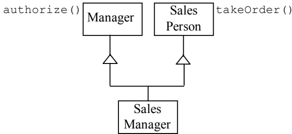
Figure 6-11: Class hierarchy for SalesManager .
