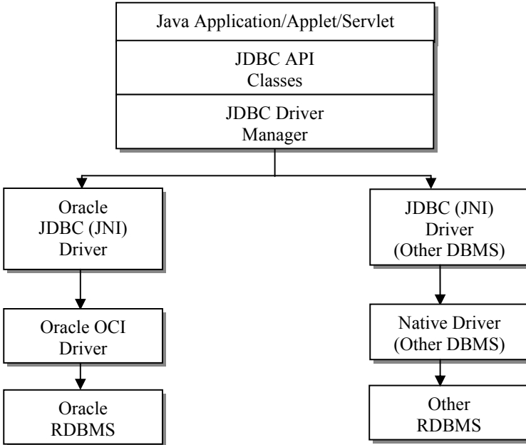
Figure 17-3: Type 2 JDBC drivers.
