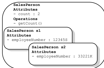
Figure 8-3: Class Method getCount()
