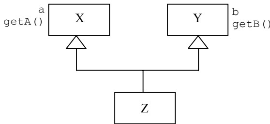
Figure 6-17: No inheritance conflict.
