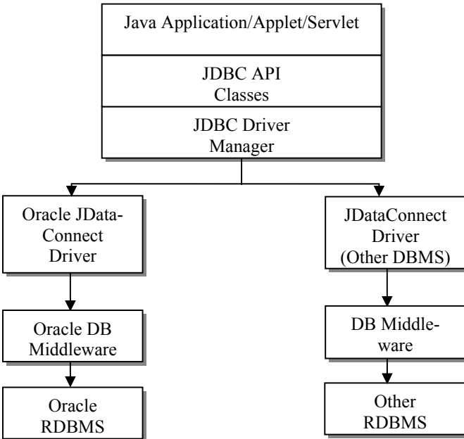
Figure 17-4: Type 3 JDBC drivers.
