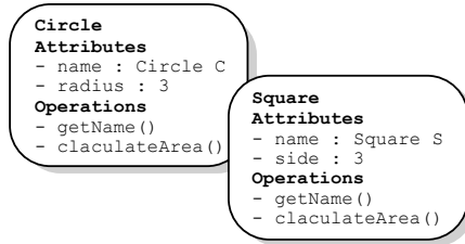
Figure 6-8: State of Circle and Square object.
