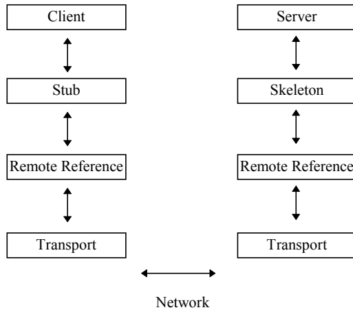
Figure 16-2: Java RMI architecture.
