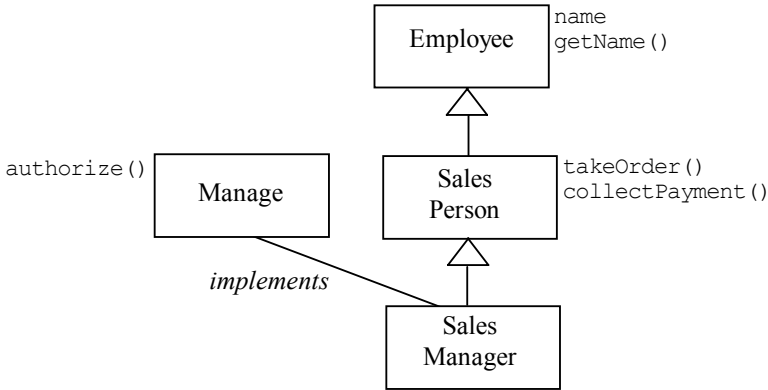
Figure 6-15: Single inheritance with interface.
