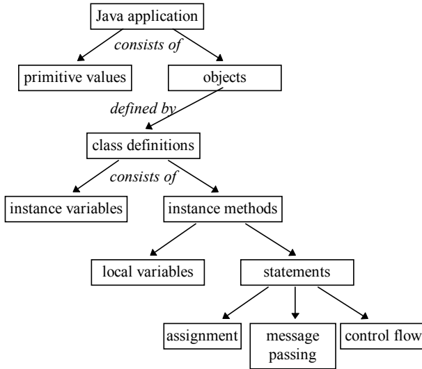
Figure 3-1: Hierarchical relationships of Java constructs.
