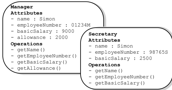
Figure 6-4: State of Manager and Secretary object.
