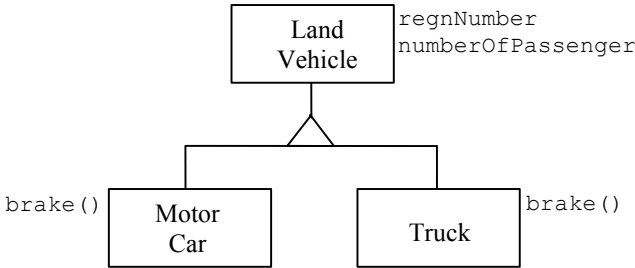
Figure 6-18: Motor car and truck.
