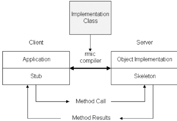
Figure 16-1: Java remote method invocation.
