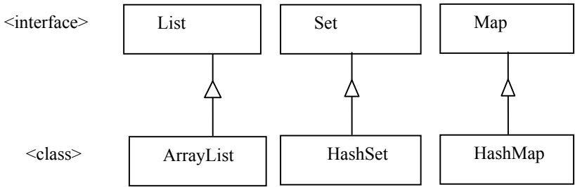
Figure 12-2: Commonly used Collection classes.
