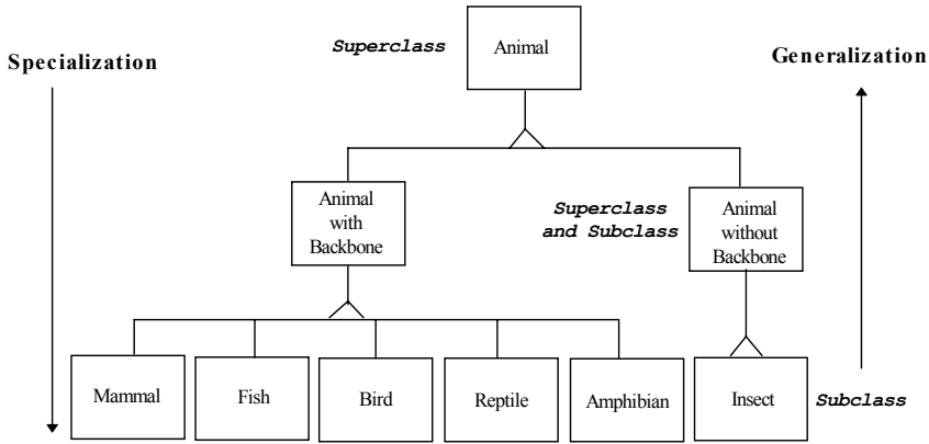
Figure 5-5: A class hierarchy for animals.
