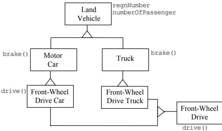
Figure 6-21: “Multiple inheritance” representation scheme.
