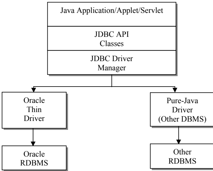
Figure 17-5: Type 4 JDBC drivers.
