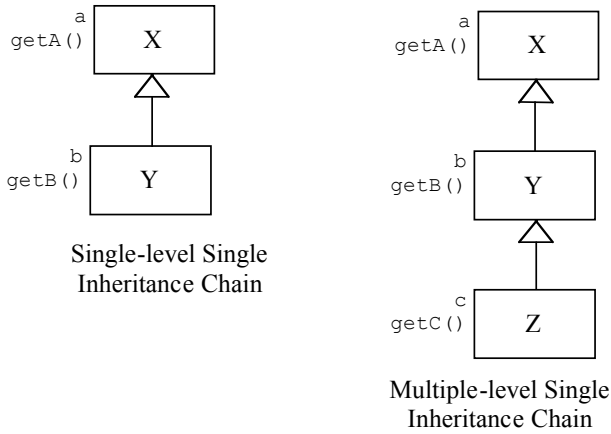
Figure 6-9: Single- and multiple-level single inheritance chains.
