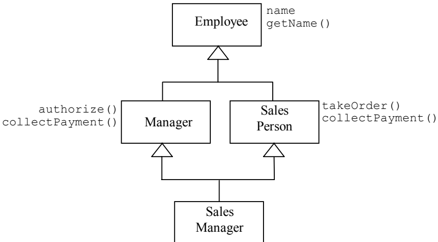
Figure 6-14: Extended class hierarchy for SalesManager .
