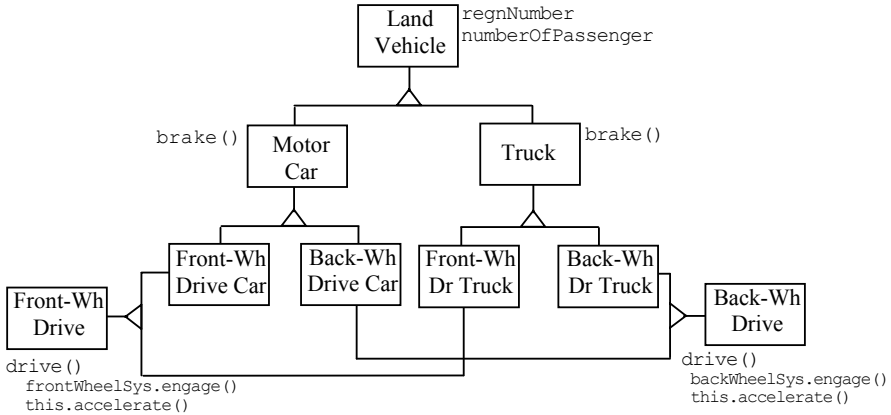
Figure 6-22: Front-Wheel and Back-Wheel Drive vehicles.
