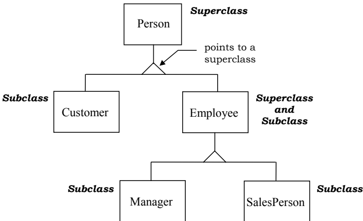
Figure 5-3: A class hierarchy diagram.
