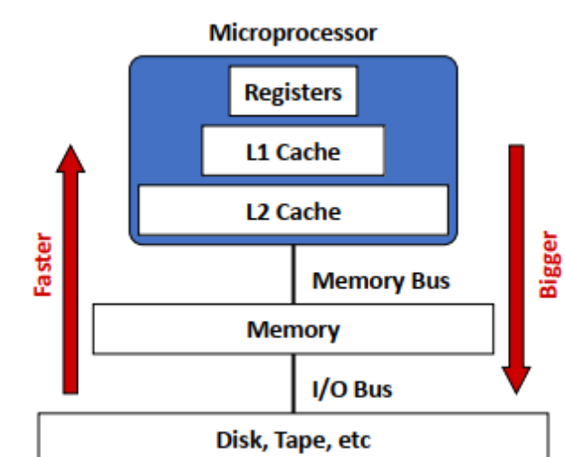
memory hierarchy
