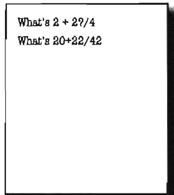
MyText.txt
