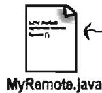
MyRemote.java
